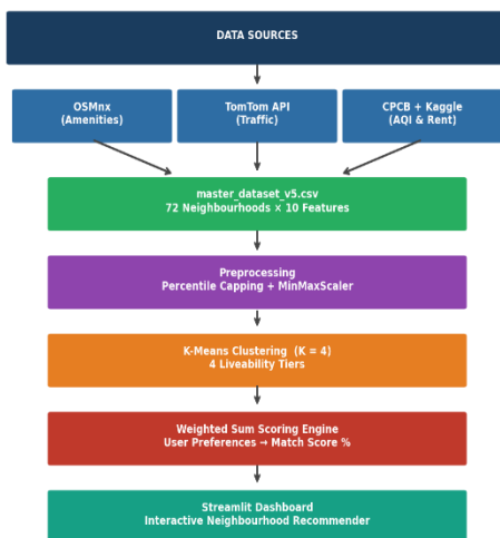
Fig. 1: CityMatch Data Pipeline
